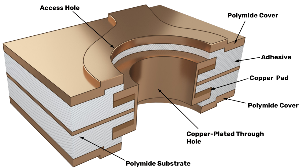
Double-sided flex circuit board
